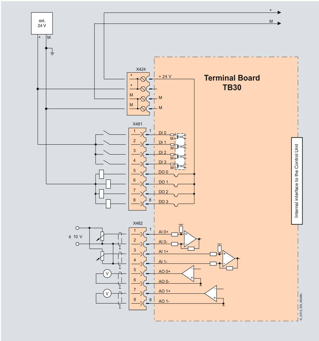
Typical connection of TB30 Terminal Board
