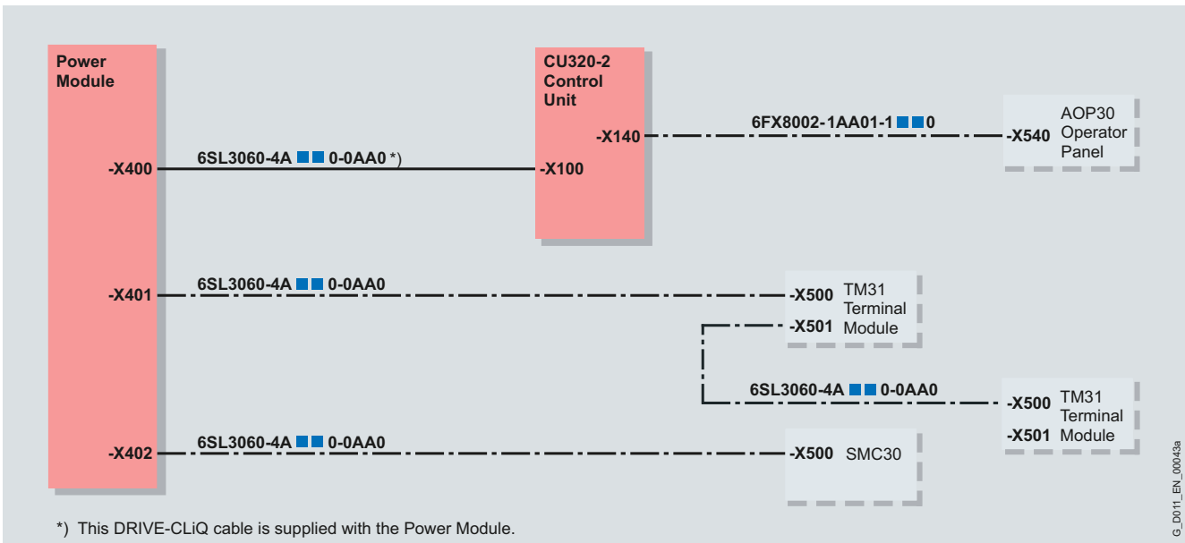
Connection example for a CU320-2 Control Unit
